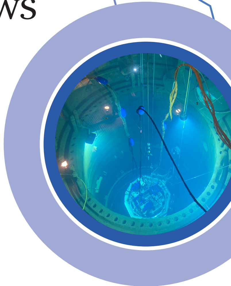
Earlier this year, the Orano segmentation team at Vermont Yankee had progressed down to the Core Shroud level in the reactor pressure vessel. Source: Orano USA.
