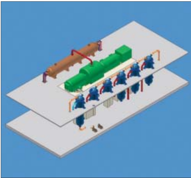
Isometric and side views of the turbine generator building barge (Source: Westinghouse Electric Co.)
