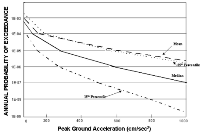
TYPICAL SEISMIC HAZARD CURVES IN THE EASTERN U.S.
