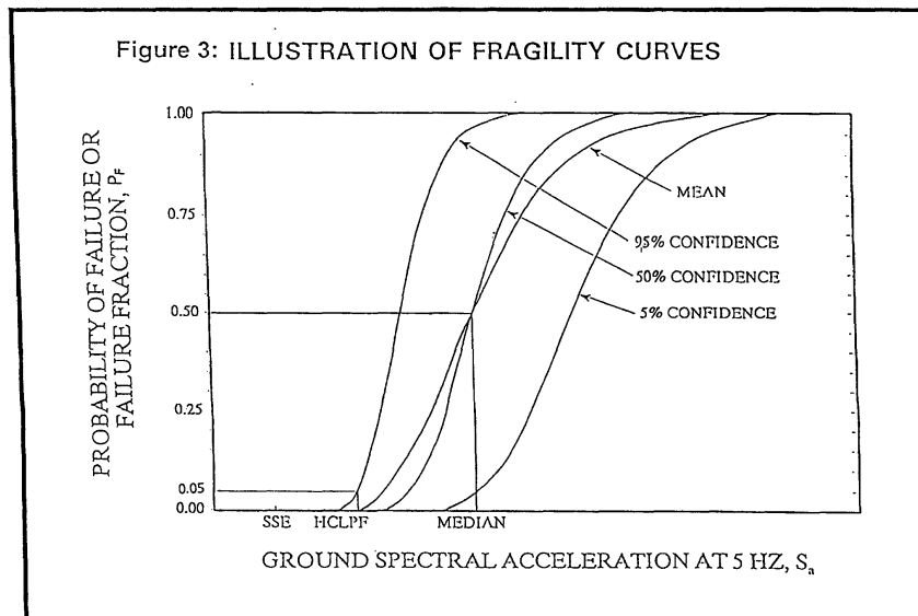
TYPICAL SEISMIC FRAGILITY CURVE(S)
